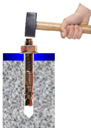
Insert assembled anchor through fixture into concrete
