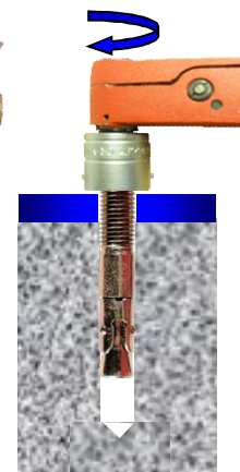
Tighten with torque wrench to recommended torque
